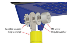
Earth connection to plates
